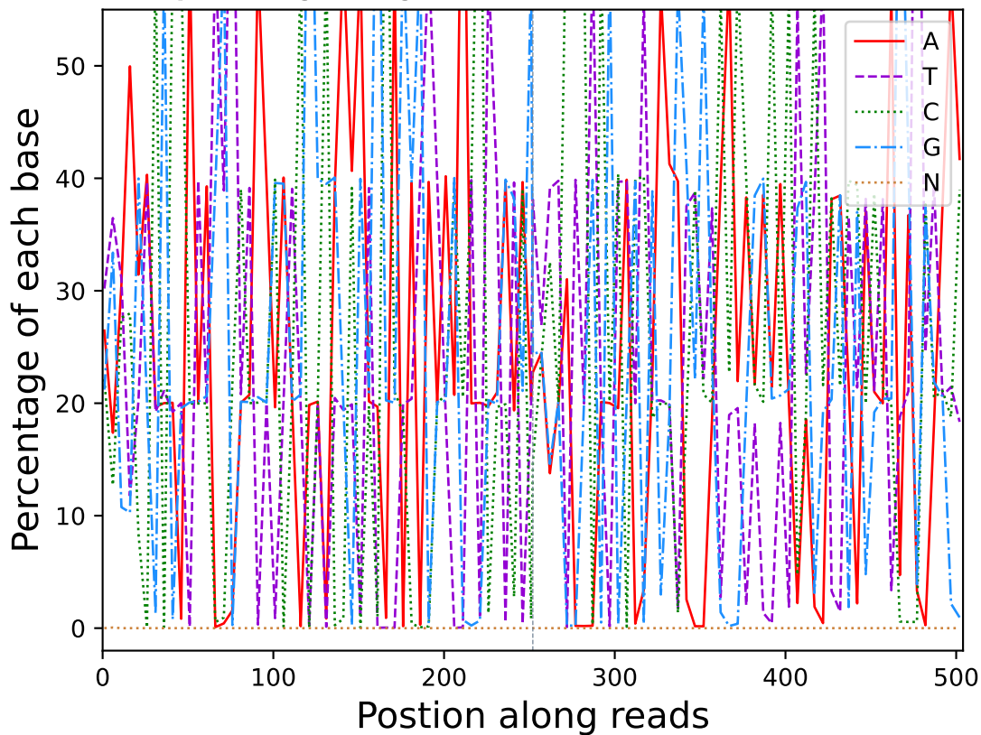
Base percentage along reads (R10722)
